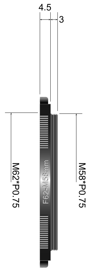
RA6258 Adapter ring
