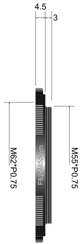
RA6255 Adapter ring
