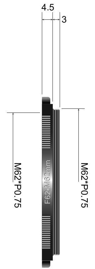
RA6262 Adapter ring
