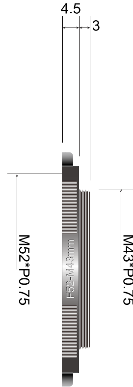
RA5243B Adapter ring
