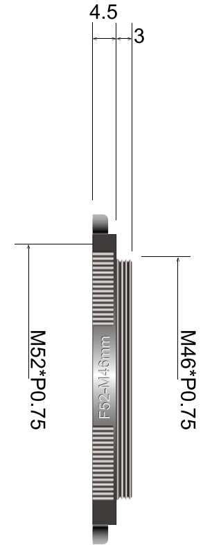
RA5246B Adapter ring
