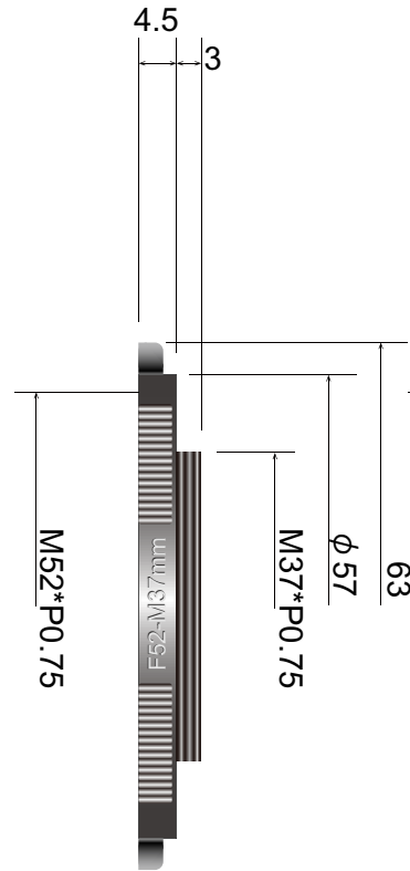
RA5237B Adapter ring
