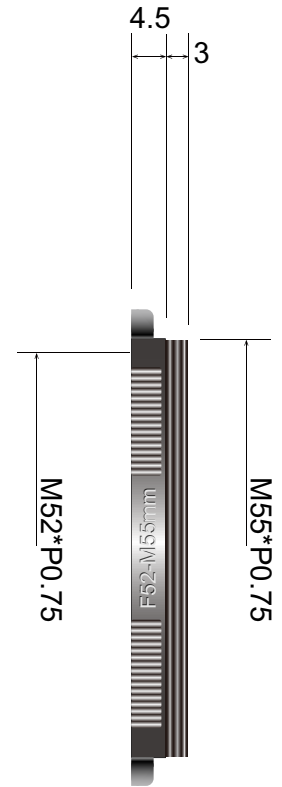
RA5255B Adapter ring
